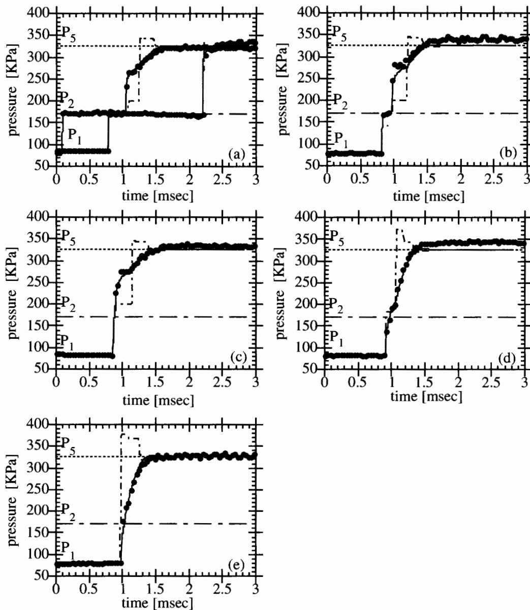
Fig. 2. Typical experimental results and their numerical simulations with a 93 mm long sample made of \text{Al}_2\text{O}_3 having 30 pores per inch (sample III in Table 1). The incident shock wave Mach number in this experiment was M_i = 1.539 (test number 13 in Table 2). The pressure histories of the pure gas just ahead of the front edge of the porous material are shown in Fig. 2(a). The pressure histories of the gas occupying the pores of the porous material along the shock tube side-wall and at its end-wall are shown in Fig. 2(b)–(e), respectively. The symbols represent the experimental results, the solid lines are the numerically predicted values when accounting for Forchheimer terms and the dash-dot lines represent the simulations without Forchheimer terms. P_1 , P_2 , and P_5 are defined in the caption of Fig. 1.
